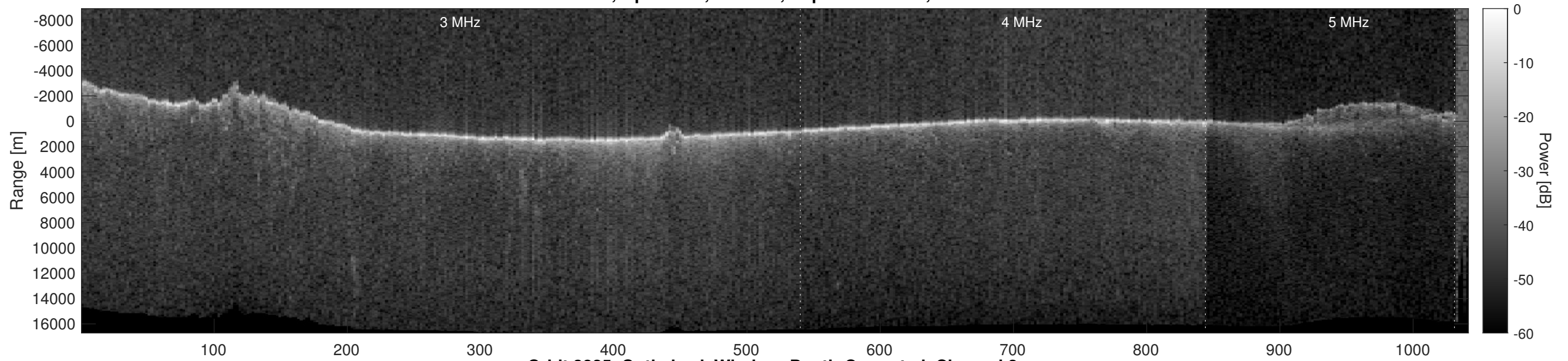
Orbit 3825, Optimized, Window, Depth-Corrected, Channel 2
