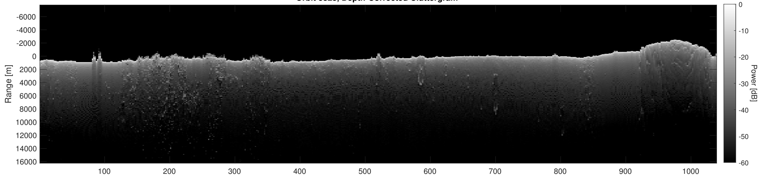
Orbit 3828, Depth-Corrected Cluttergram
