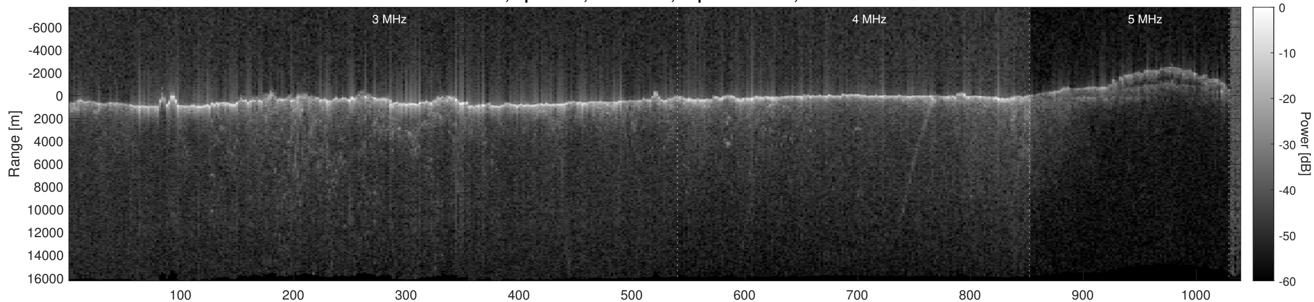
Orbit 3828, Optimized, No Window, Depth-Corrected, Channel 2
