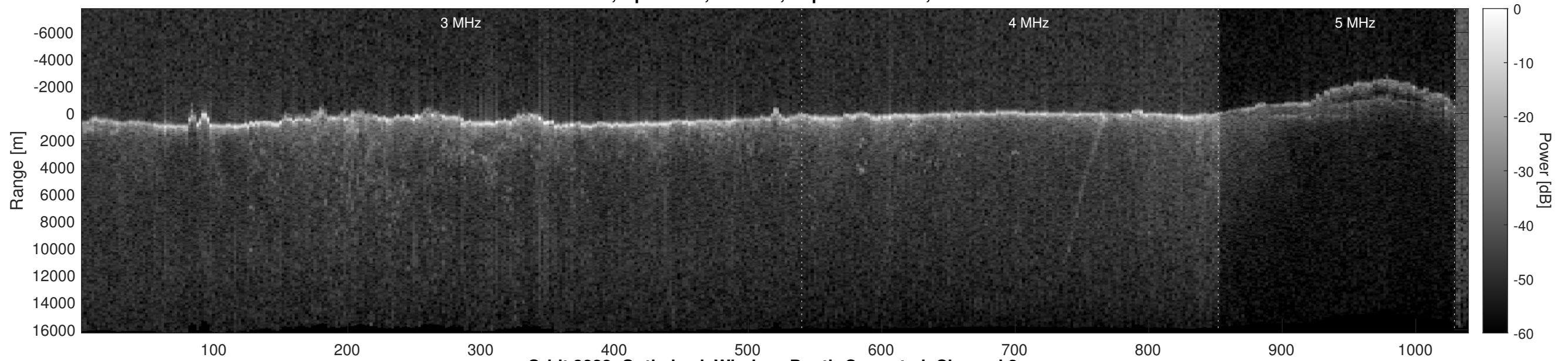
Orbit 3828, Optimized, Window, Depth-Corrected, Channel 2
