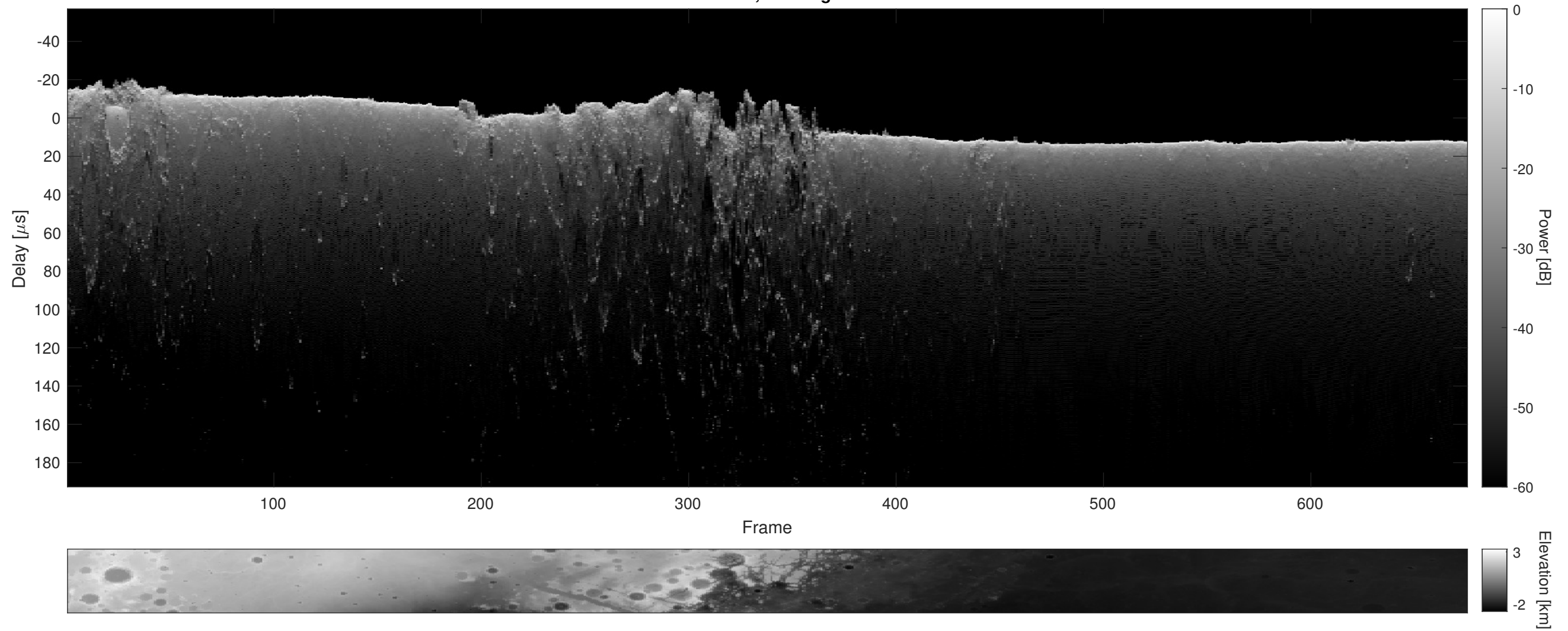
Orbit 3829, Cluttergram
