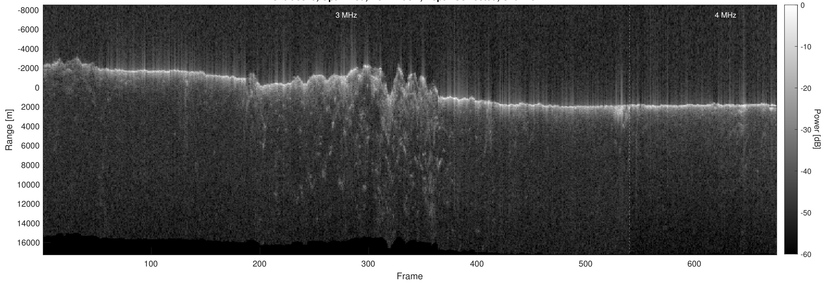
Orbit 3829, Optimized, No Window, Depth-Corrected, Channel 2
