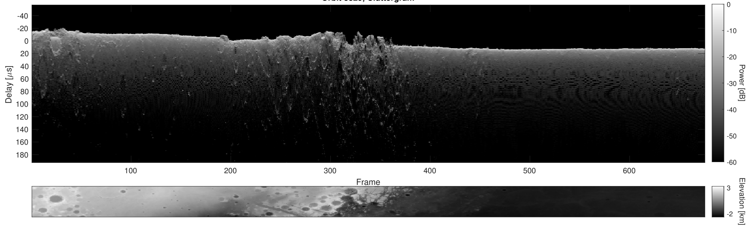
Orbit 3829, Cluttergram
