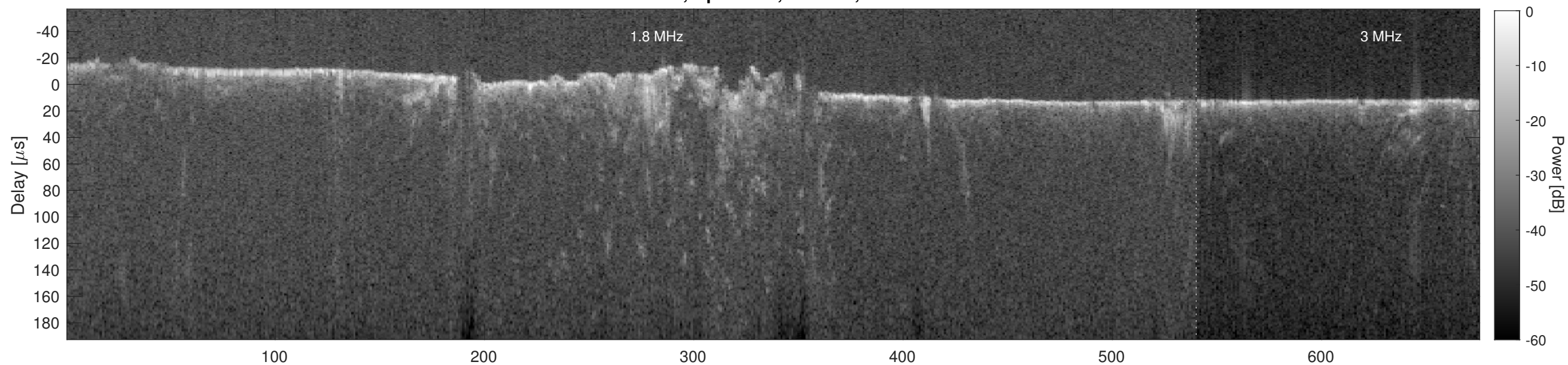
Orbit 3829, Cluttergram
