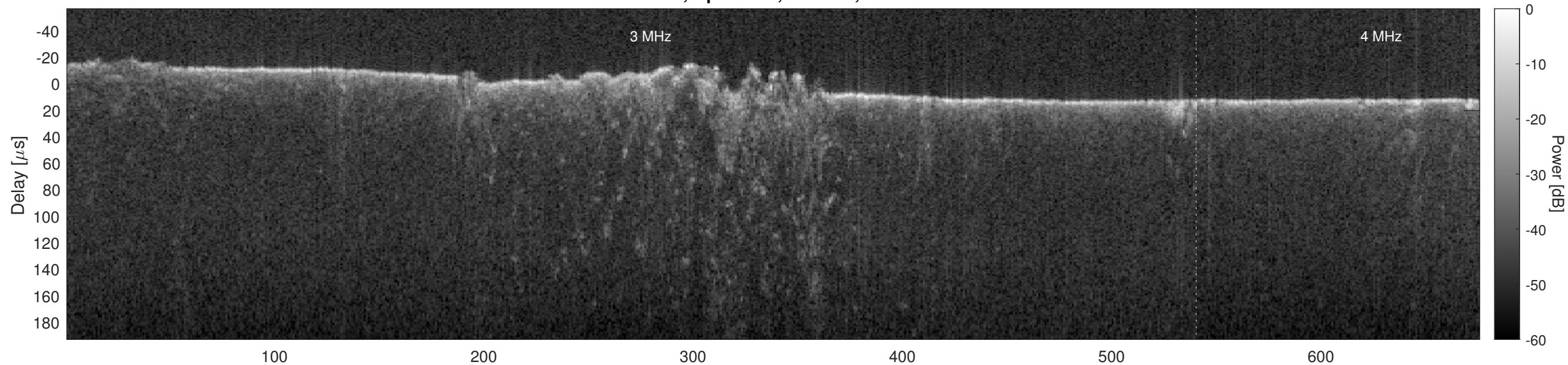
Orbit 3829, Optimized, Window, Channel 2
