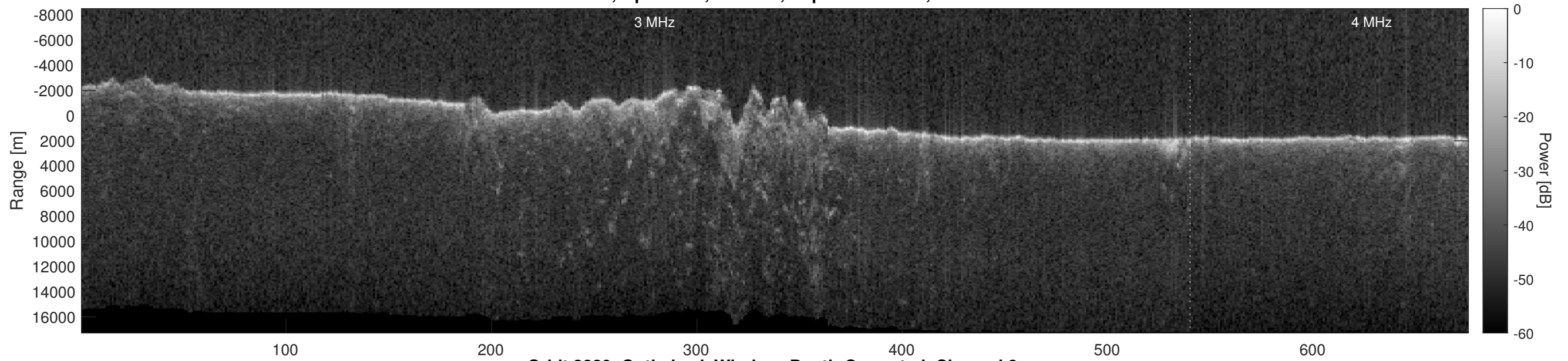
Orbit 3829, Optimized, Window, Depth-Corrected, Channel 2
