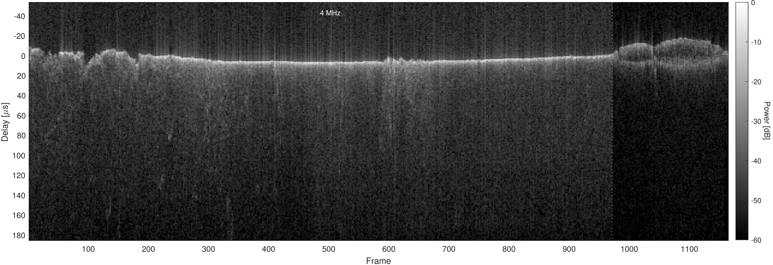
Orbit 3830, Optimized, No Window, Channel 2
