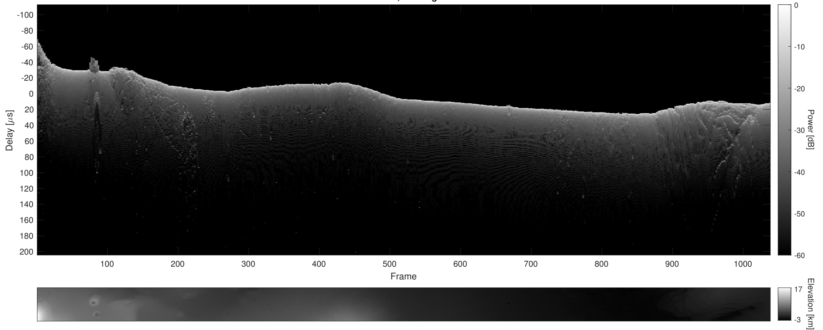
Orbit 3831, Cluttergram
