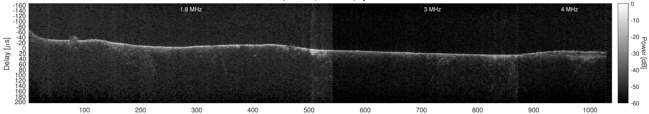
Orbit 3831, Cluttergram
