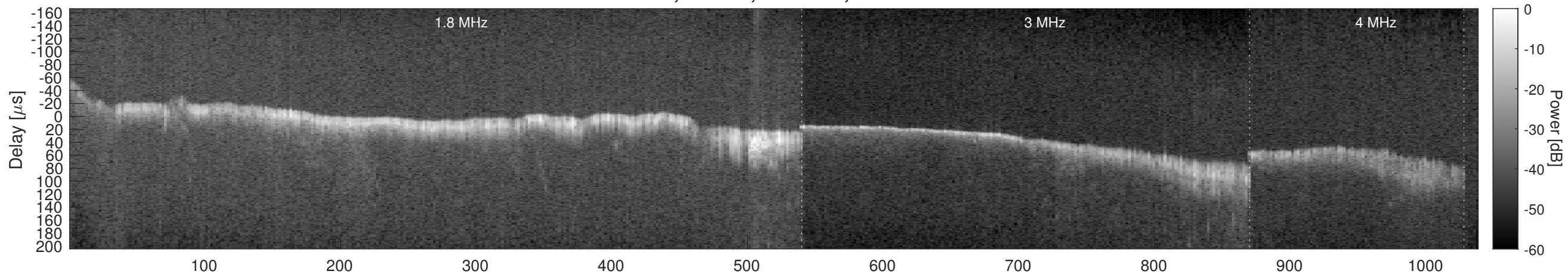
Orbit 3831, Window, Channel 2, Chapman
