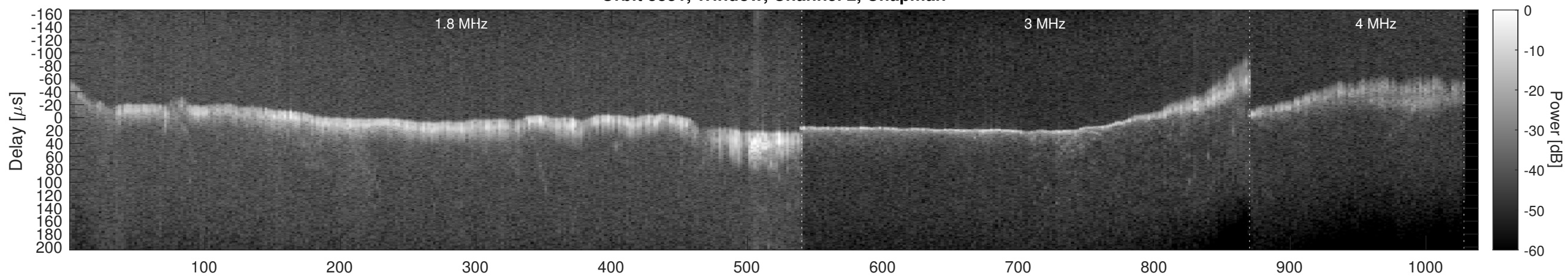
Orbit 3831, Window, Channel 2, Optimized
