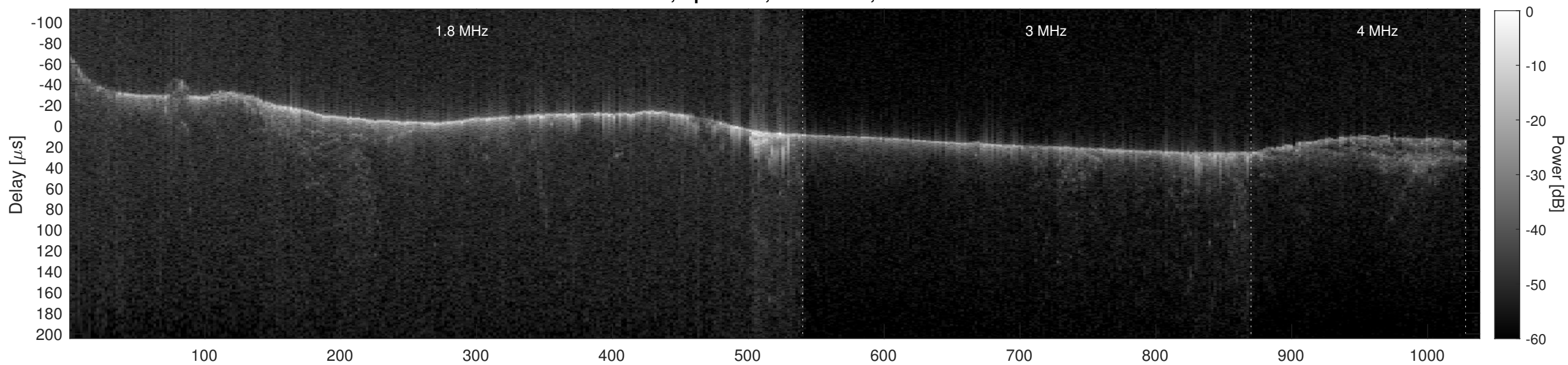
Orbit 3831, Cluttergram
