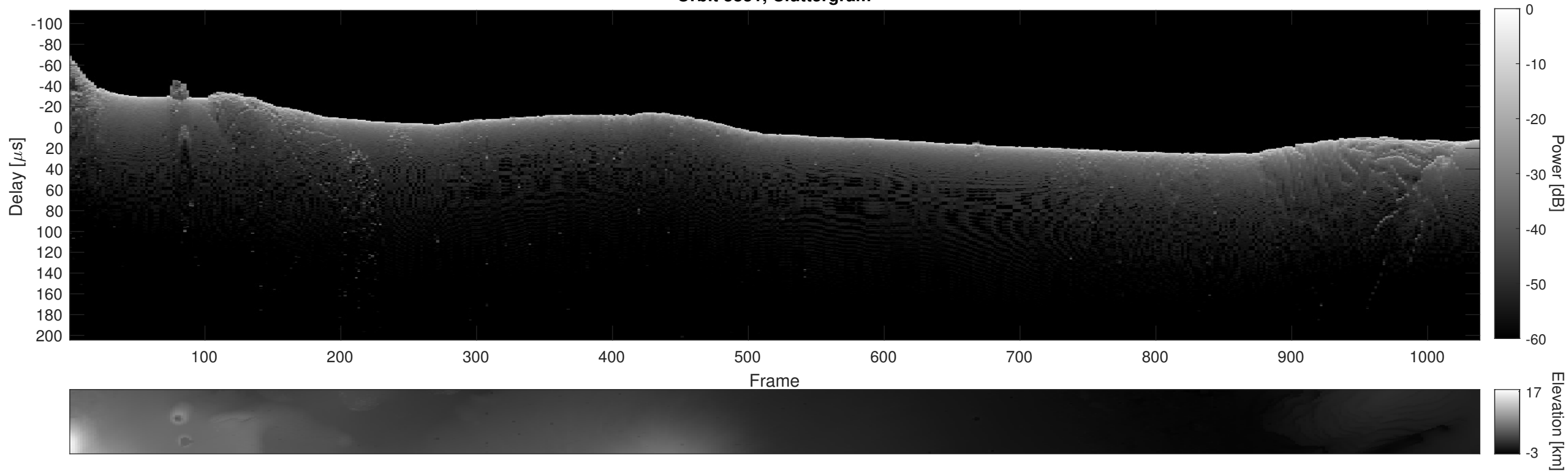
Orbit 3831, Cluttergram
