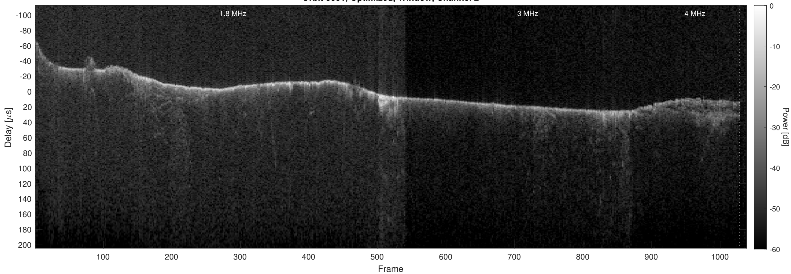
Orbit 3831, Optimized, Window, Channel 2
