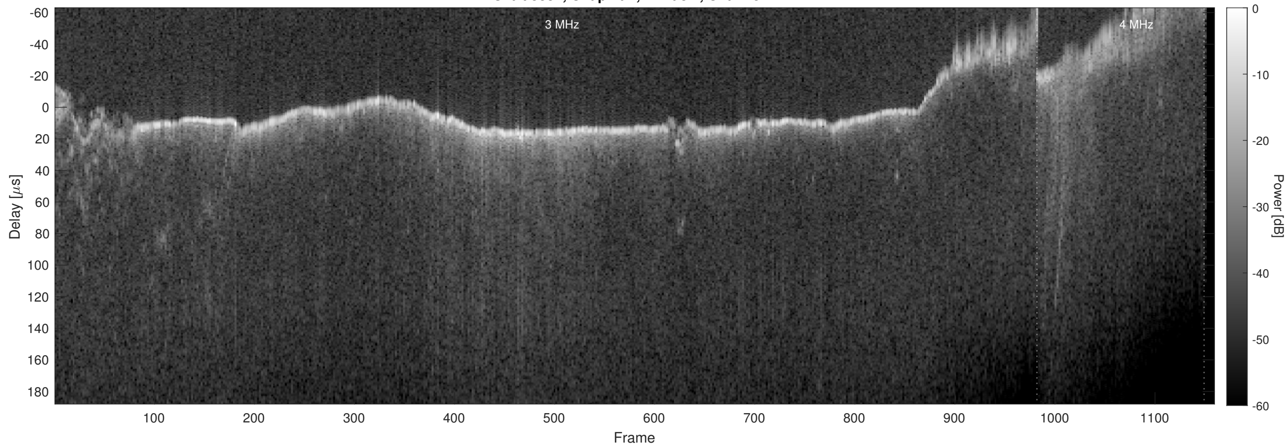
Orbit 3832, Chapman, Window, Channel 2
