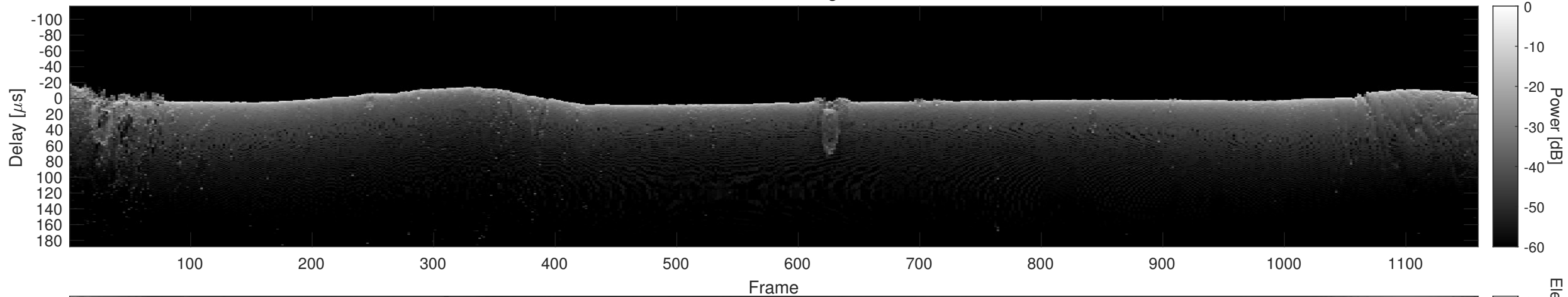
Orbit 3832, Cluttergram
