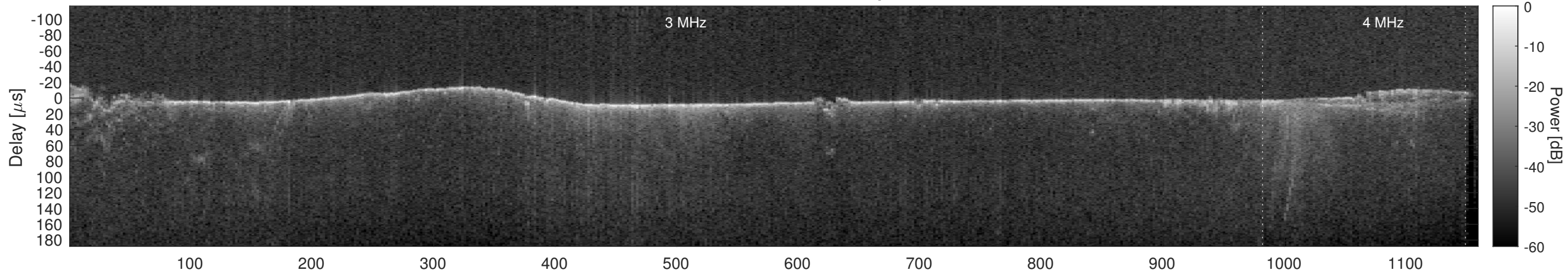
Orbit 3832, Cluttergram
