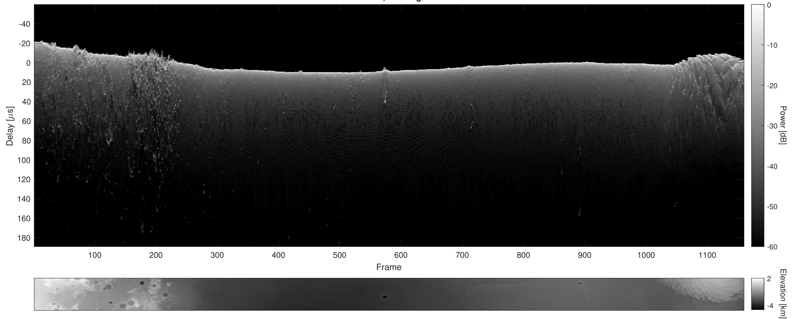
Orbit 3836, Cluttergram
