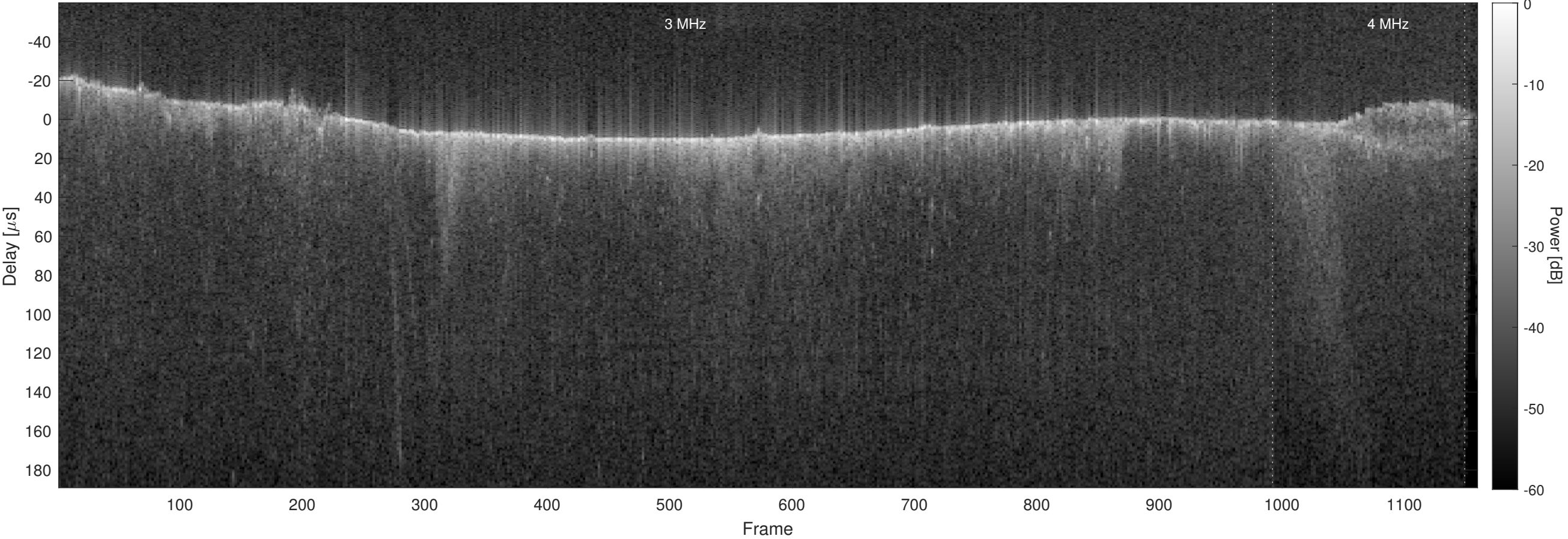
Orbit 3836, Optimized, No Window, Channel 2
