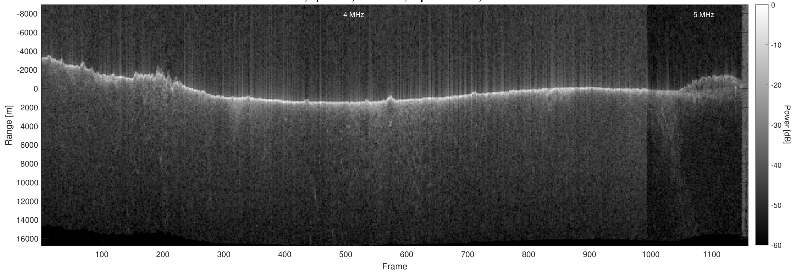
Orbit 3836, Optimized, No Window, Depth-Corrected, Channel 2
