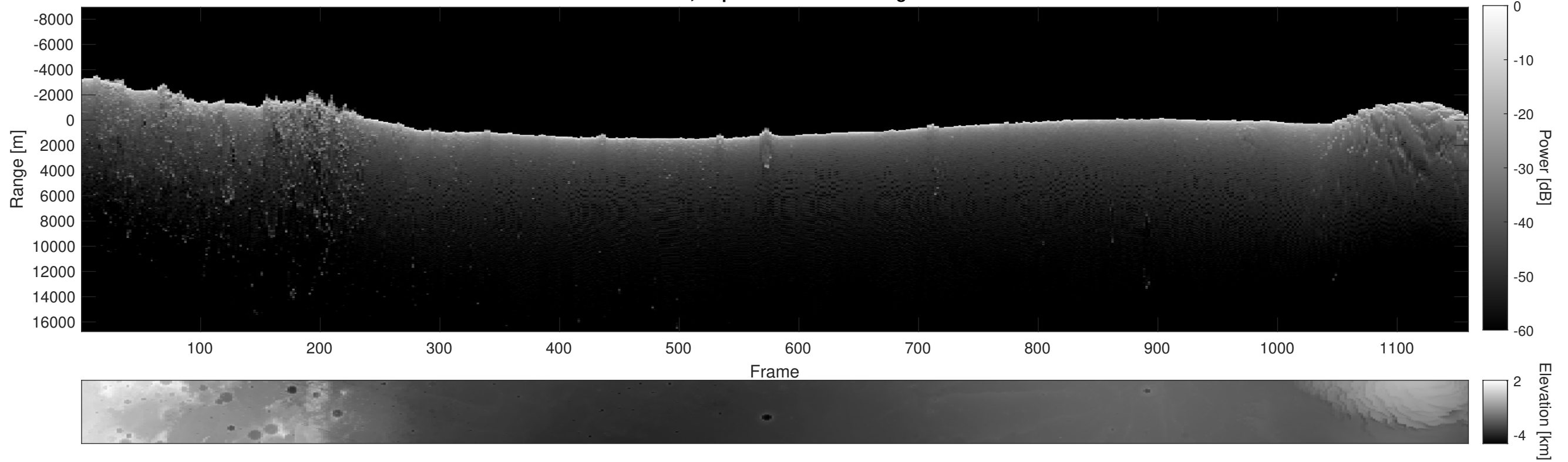
Orbit 3836, Depth-Corrected Cluttergram
