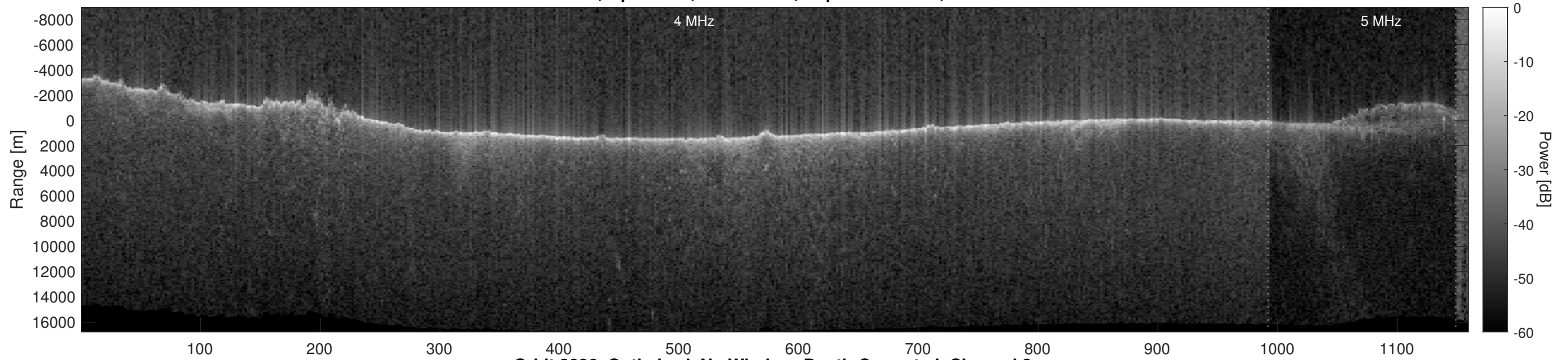
Orbit 3836, Optimized, No Window, Depth-Corrected, Channel 2
