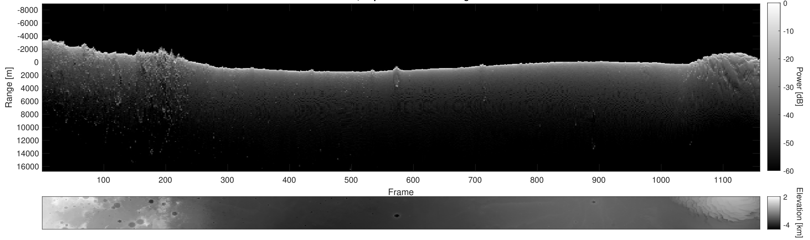
Orbit 3836, Depth-Corrected Cluttergram
