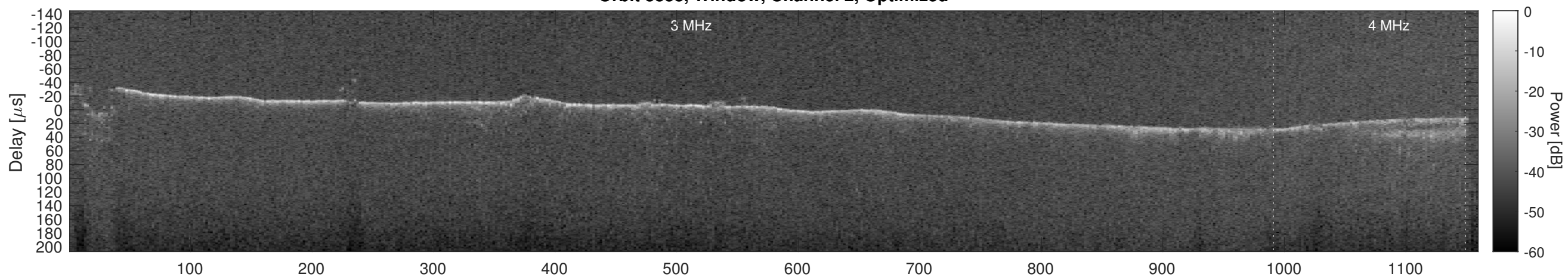
Orbit 3838, Cluttergram
