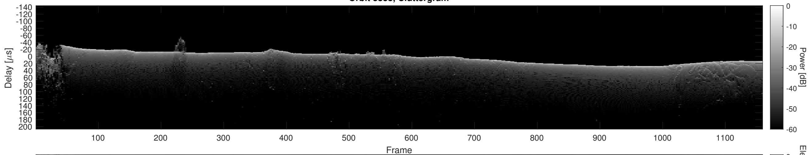
Orbit 3838, Cluttergram
