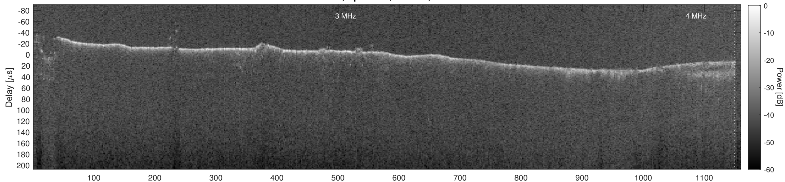
Orbit 3838, Cluttergram
