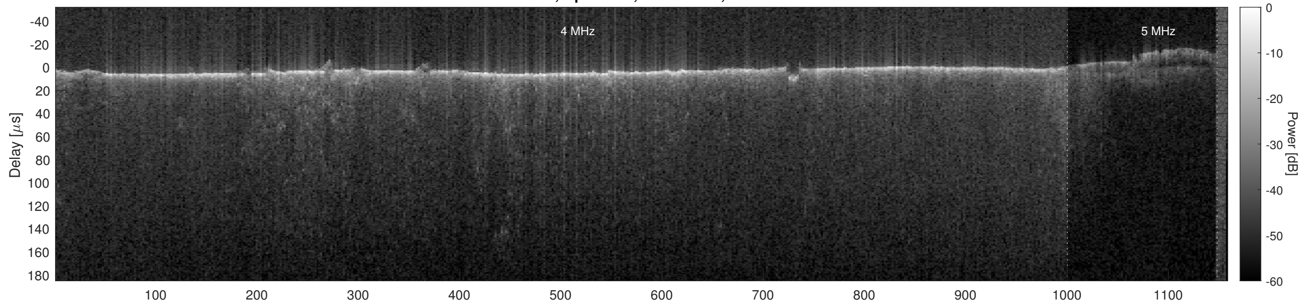
Orbit 3839, Optimized, No Window, Channel 2
