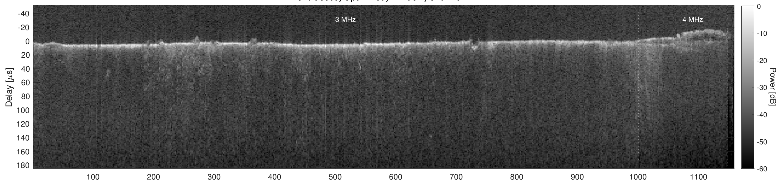
Orbit 3839, Cluttergram
