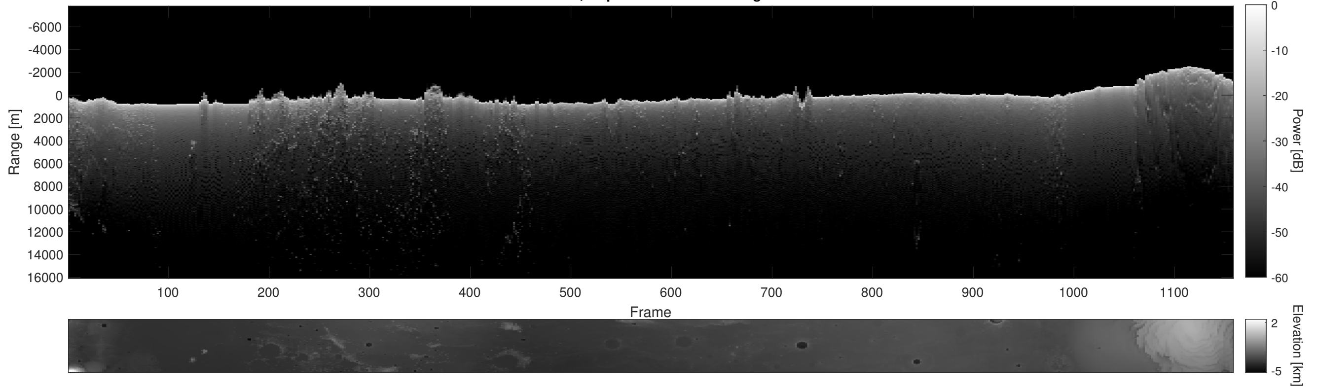
Orbit 3839, Depth-Corrected Cluttergram
