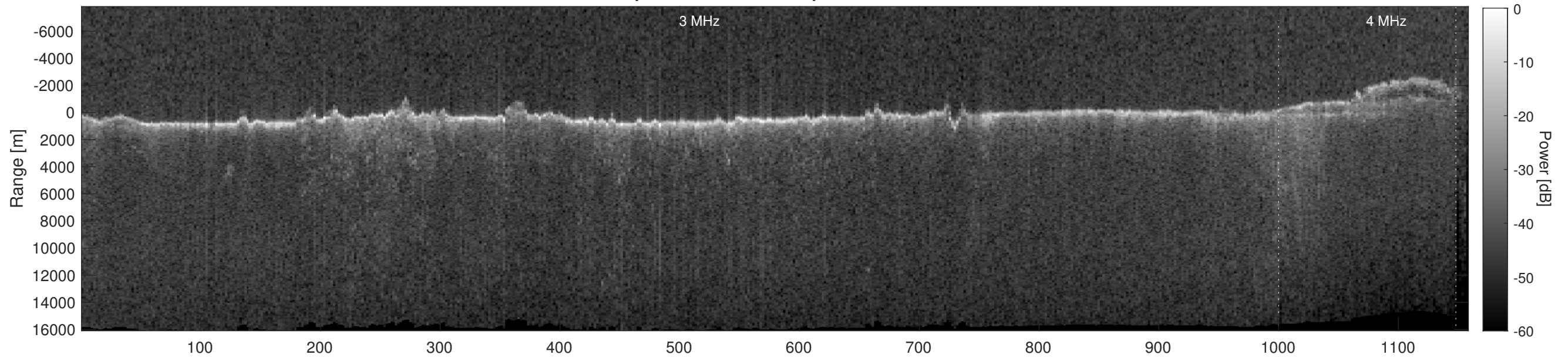
Orbit 3839, Depth-Corrected Cluttergram
