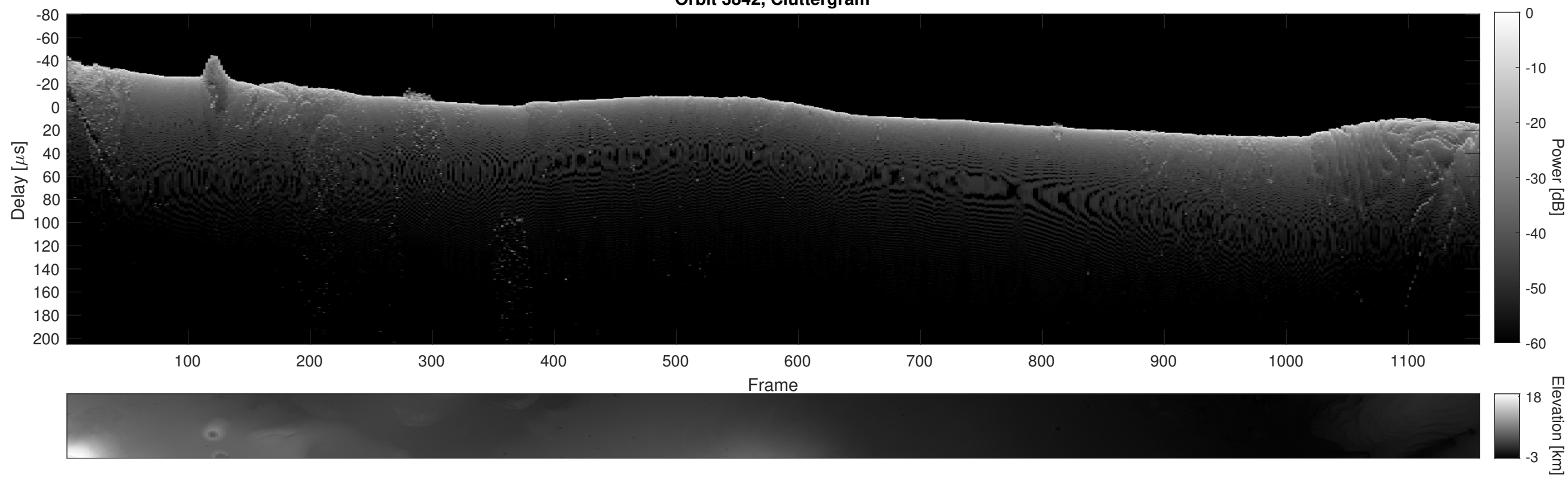
Orbit 3842, Cluttergram
