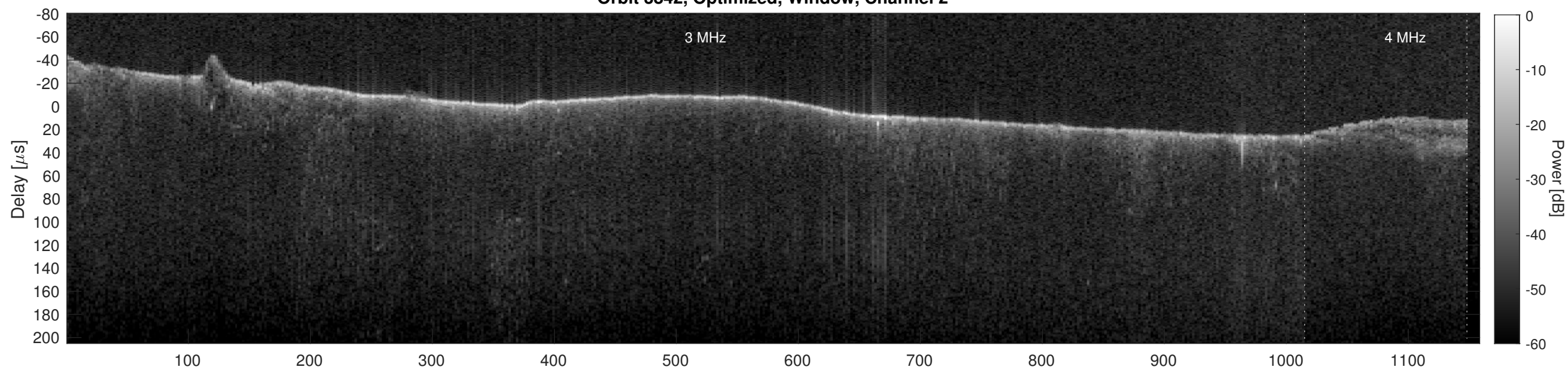
Orbit 3842, Cluttergram
