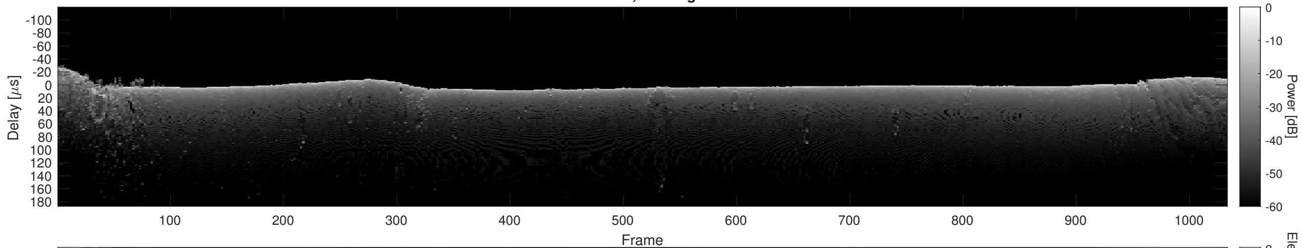
Orbit 3843, Cluttergram
