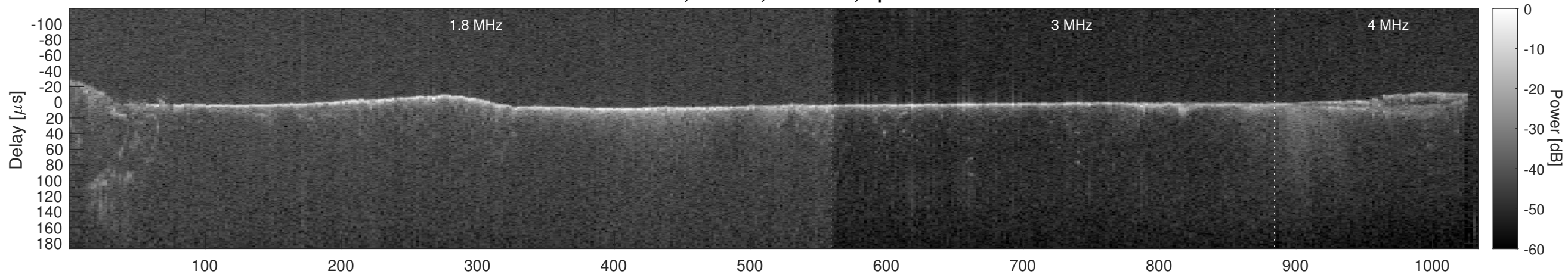
Orbit 3843, Cluttergram
