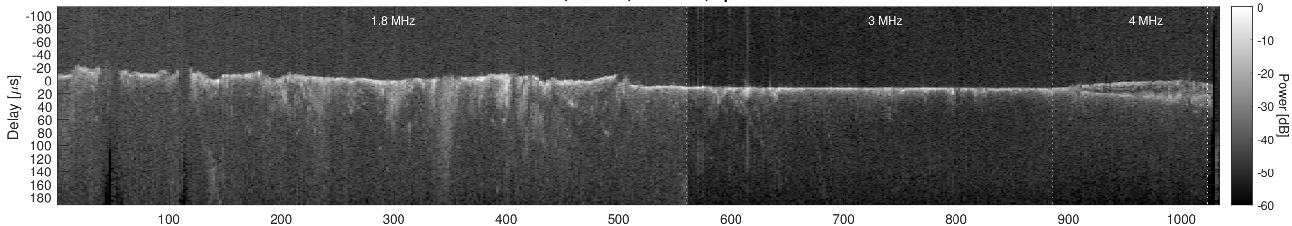
Orbit 3844, Cluttergram
