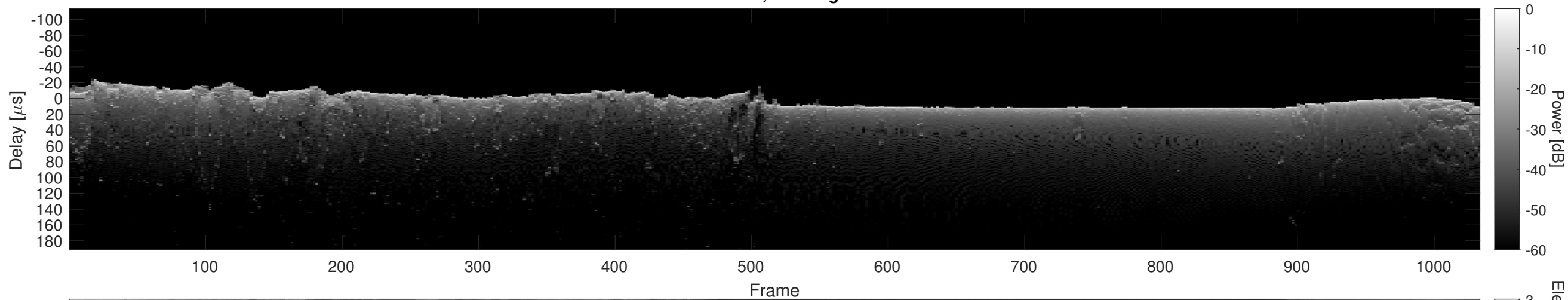
Orbit 3844, Cluttergram
