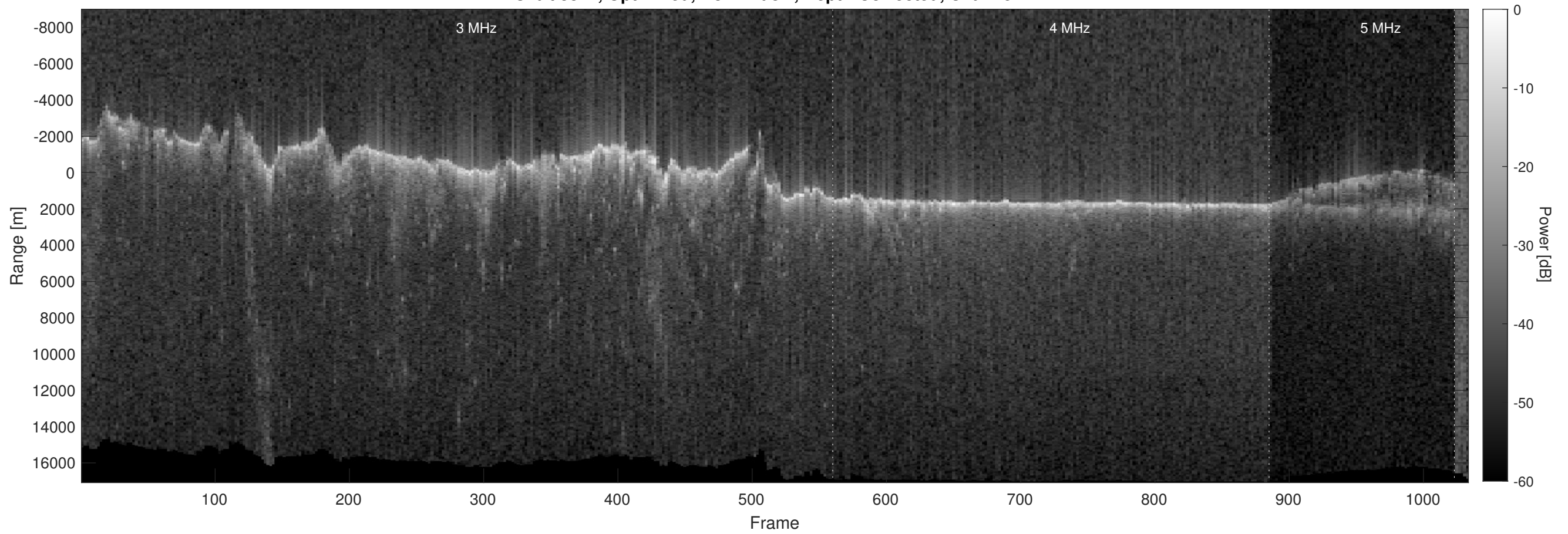
Orbit 3844, Optimized, No Window, Depth-Corrected, Channel 2
