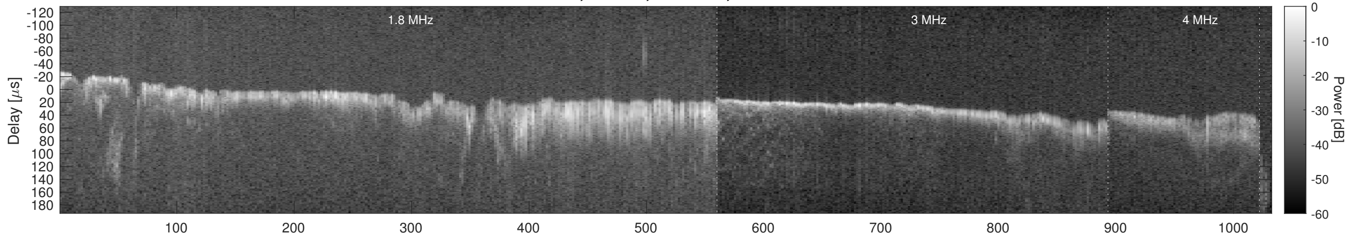
Orbit 3845, Window, Channel 2, Chapman
