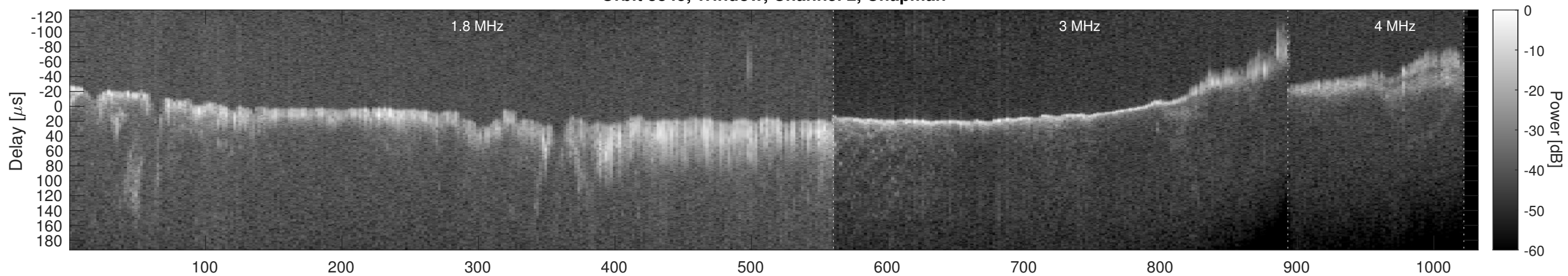
Orbit 3845, Window, Channel 2, Optimized
