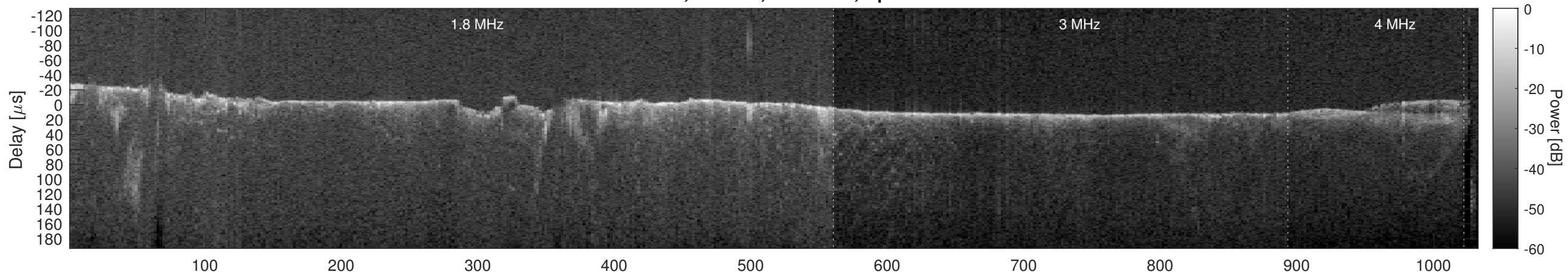
Orbit 3845, Cluttergram
