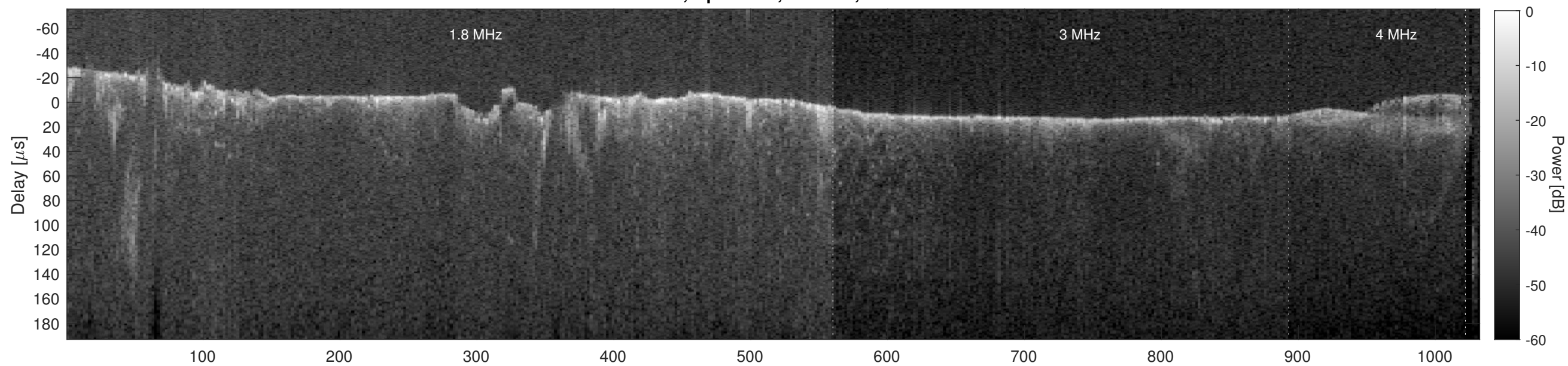
Orbit 3845, Cluttergram
