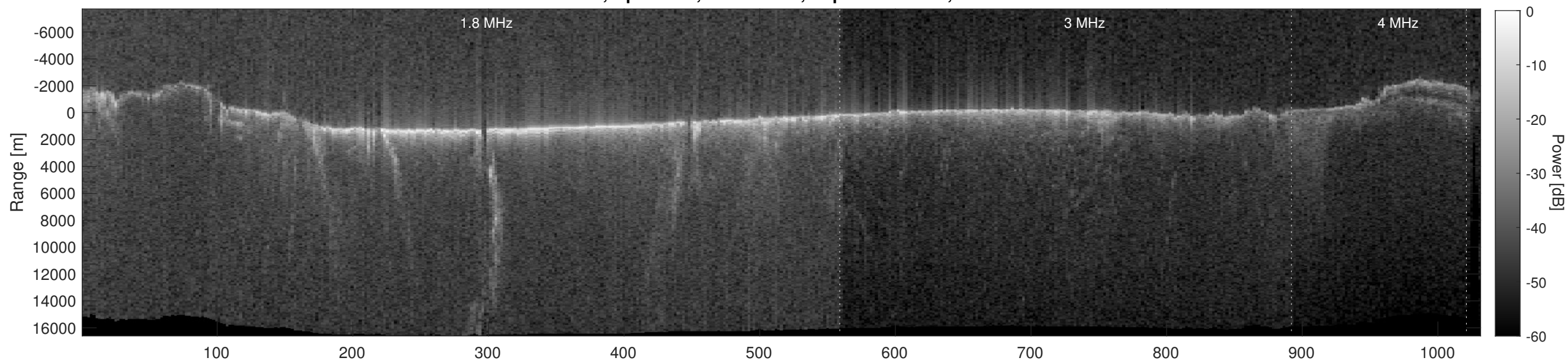
Orbit 3846, Depth-Corrected Cluttergram
