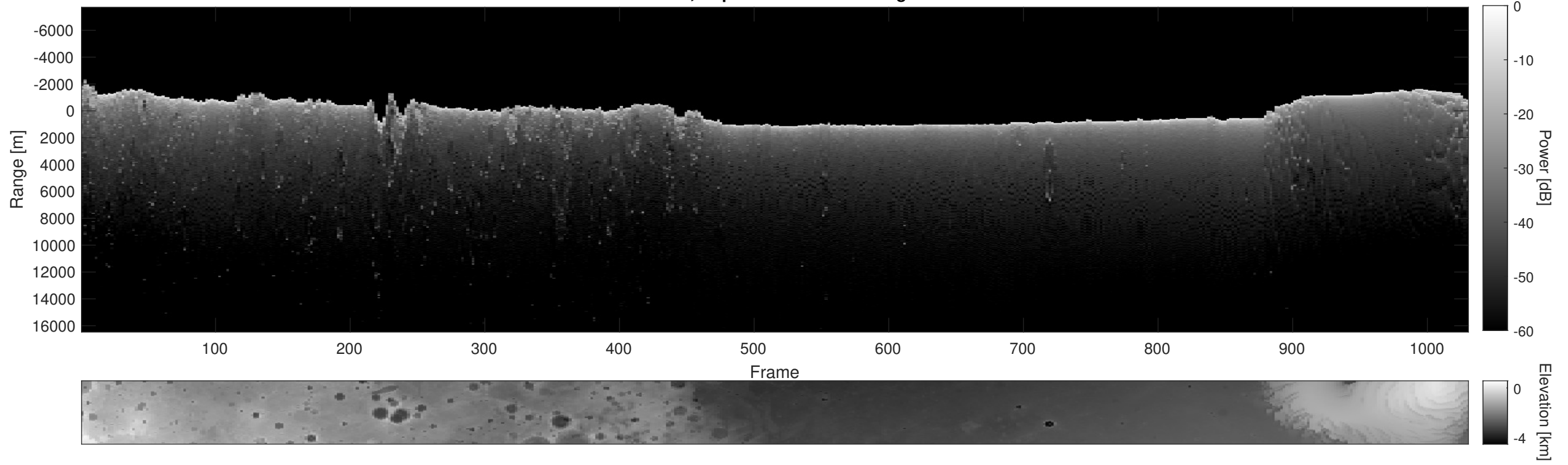
Orbit 3848, Depth-Corrected Cluttergram
