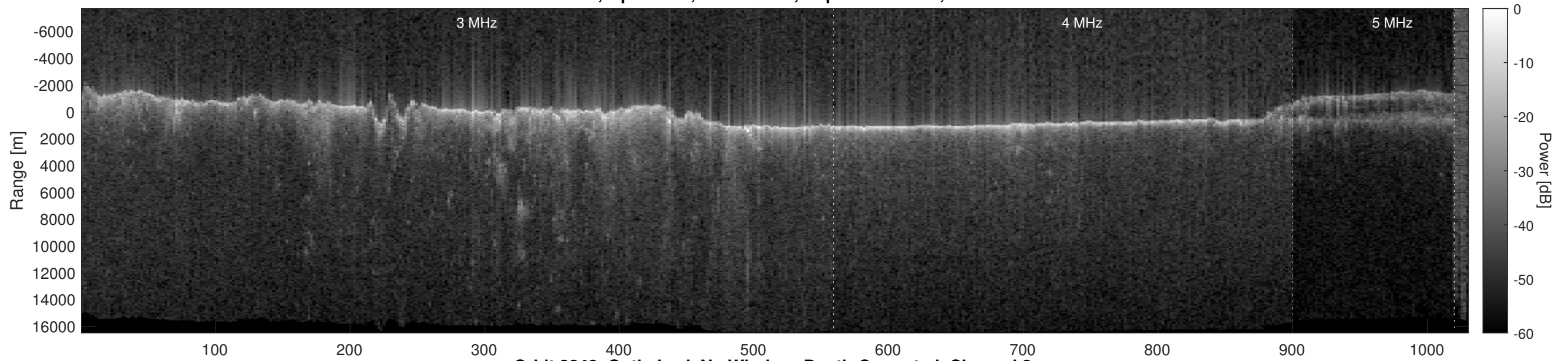
Orbit 3848, Optimized, No Window, Depth-Corrected, Channel 2
