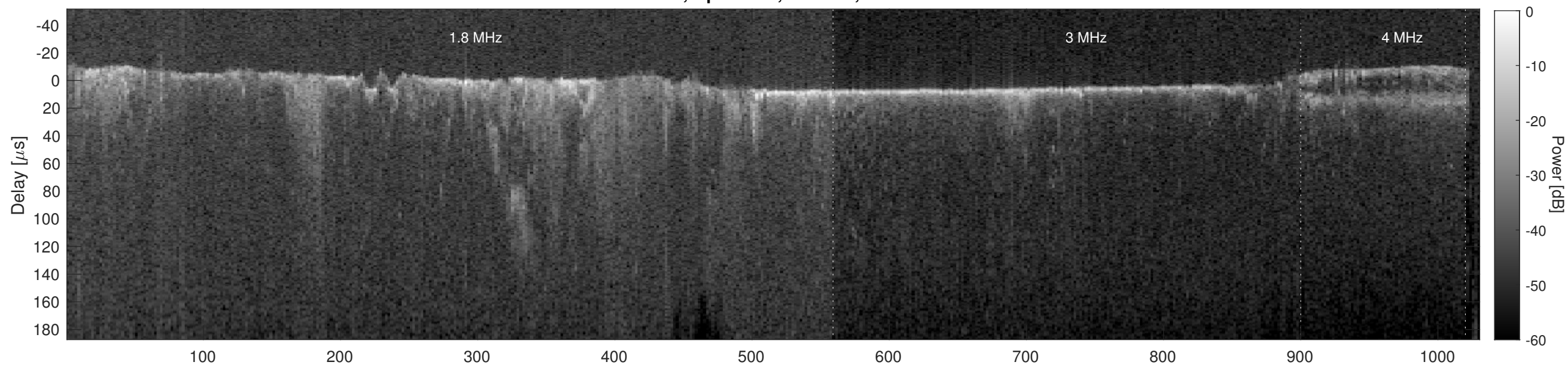
Orbit 3848, Cluttergram
