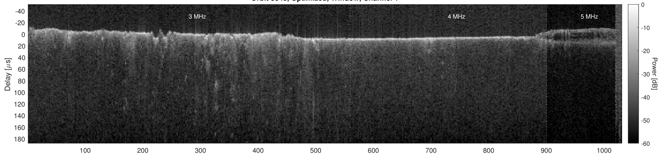
Orbit 3848, Optimized, Window, Channel 2
