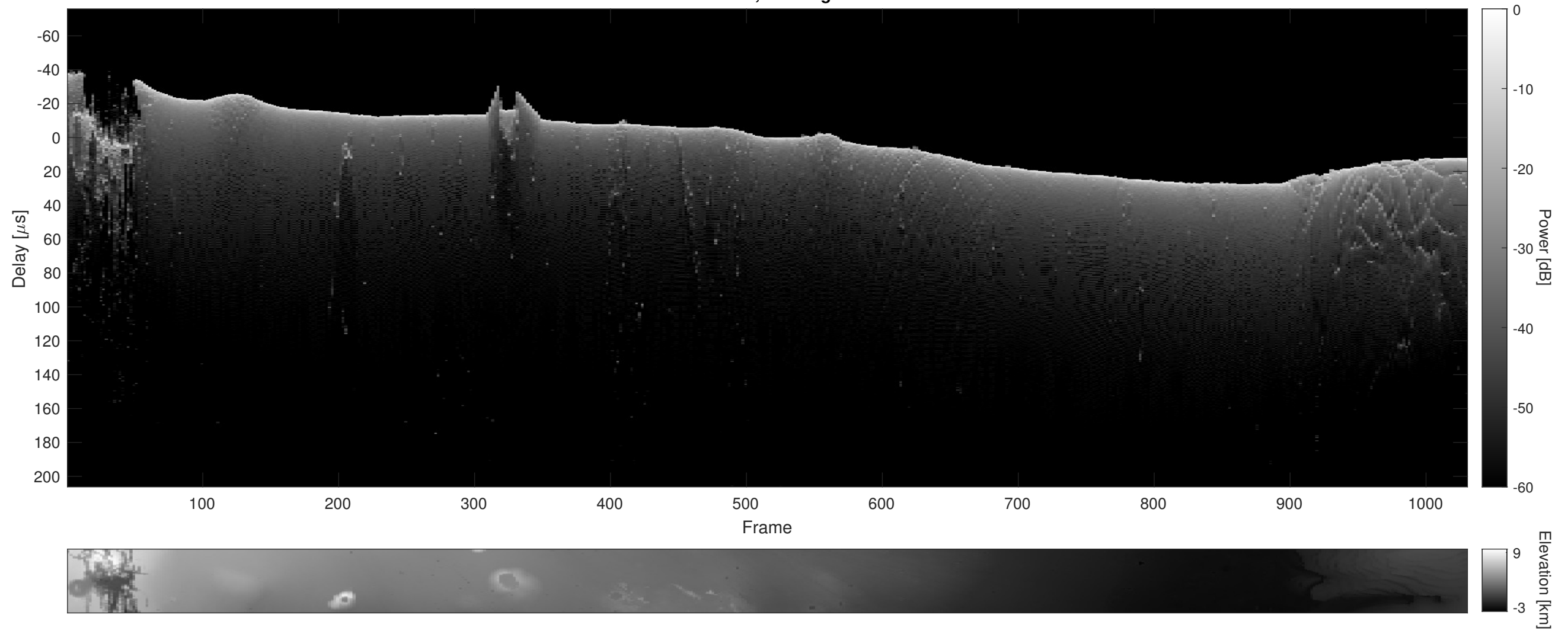
Orbit 3849, Cluttergram
