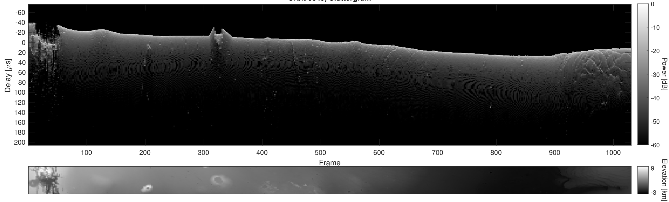
Orbit 3849, Cluttergram
