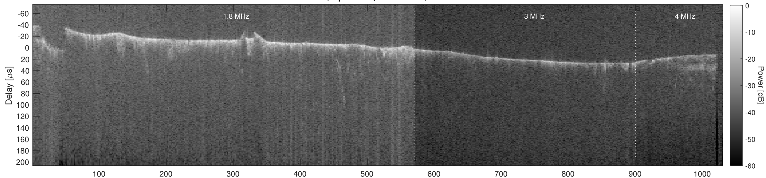
Orbit 3849, Cluttergram
