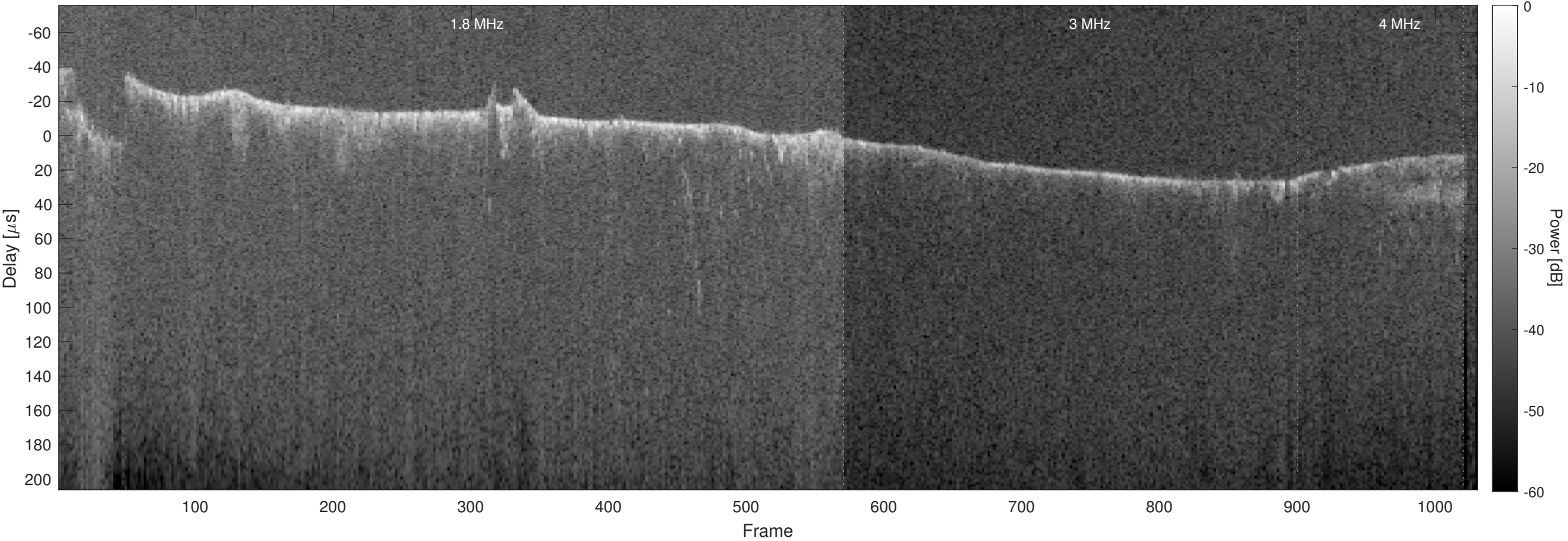
Orbit 3849, Optimized, Window, Channel 2
