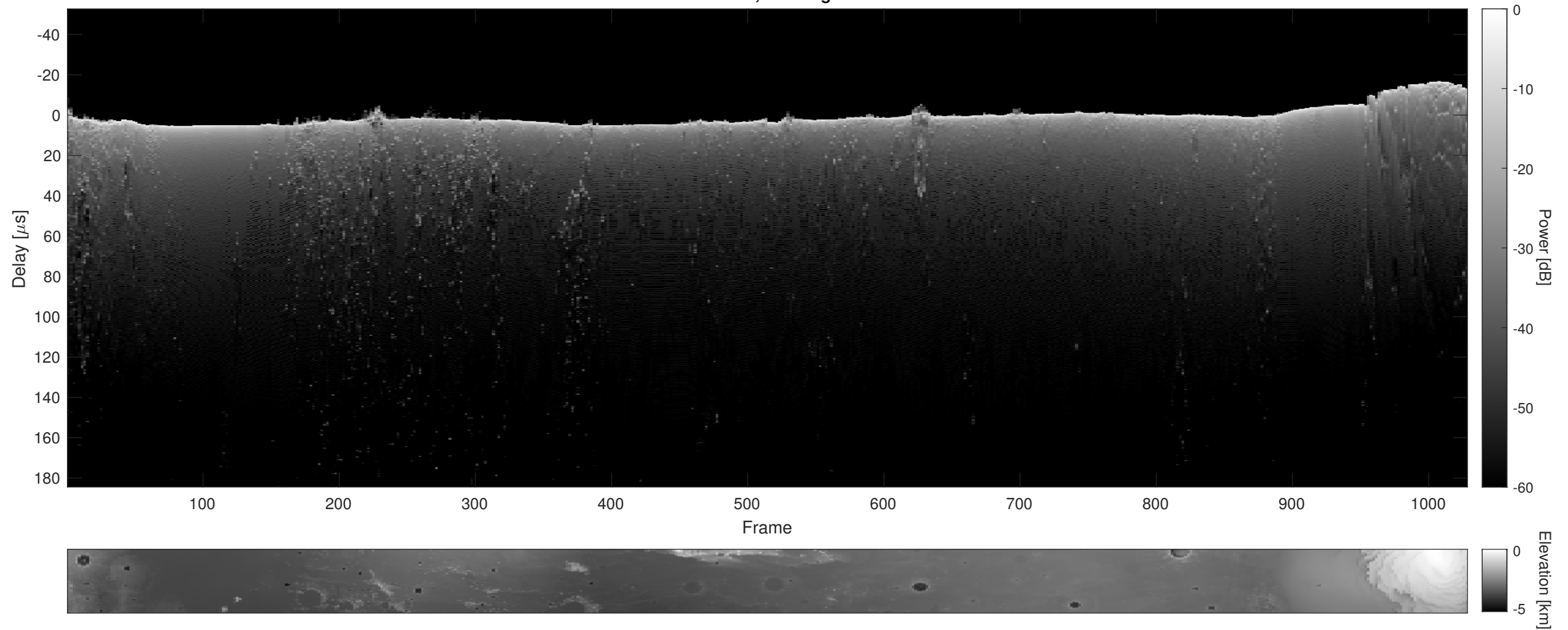
Orbit 3850, Cluttergram
