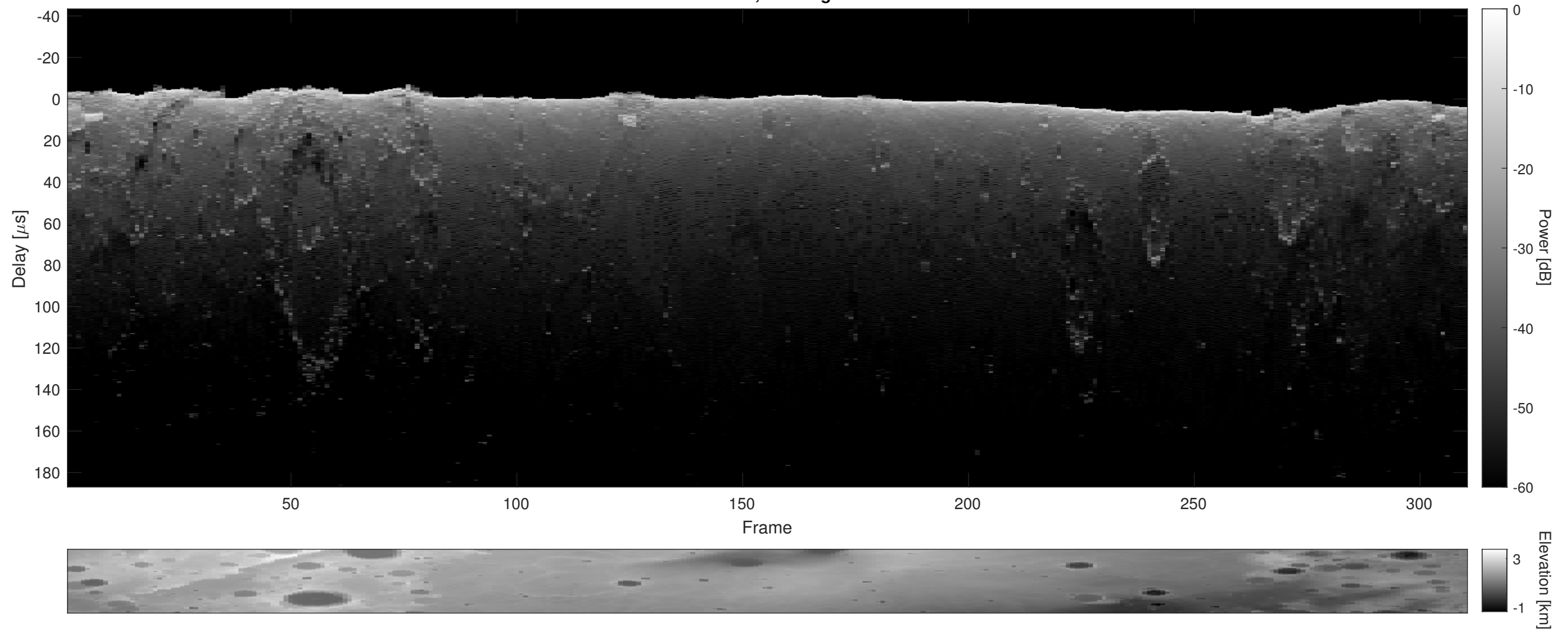
Orbit 3851, Cluttergram
