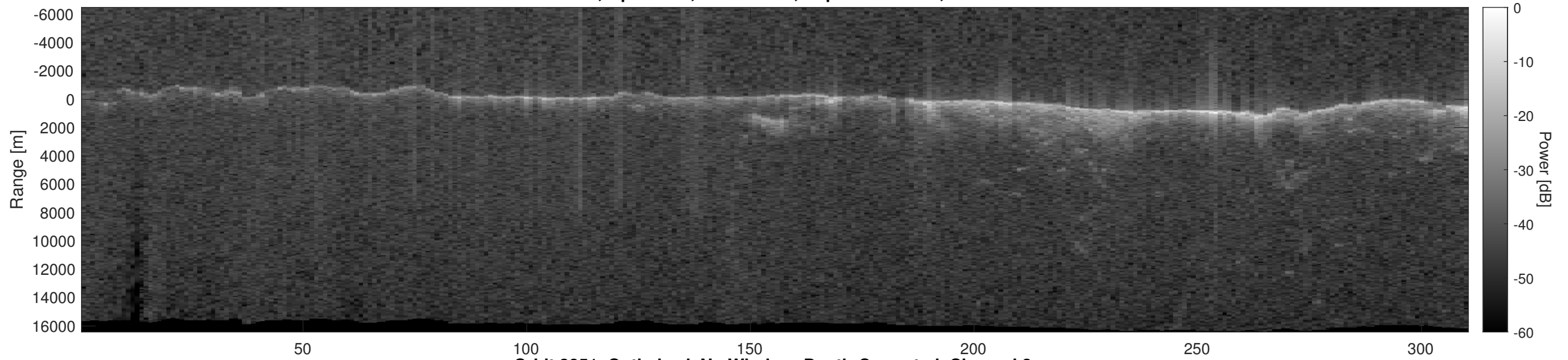
Orbit 3851, Optimized, No Window, Depth-Corrected, Channel 2
