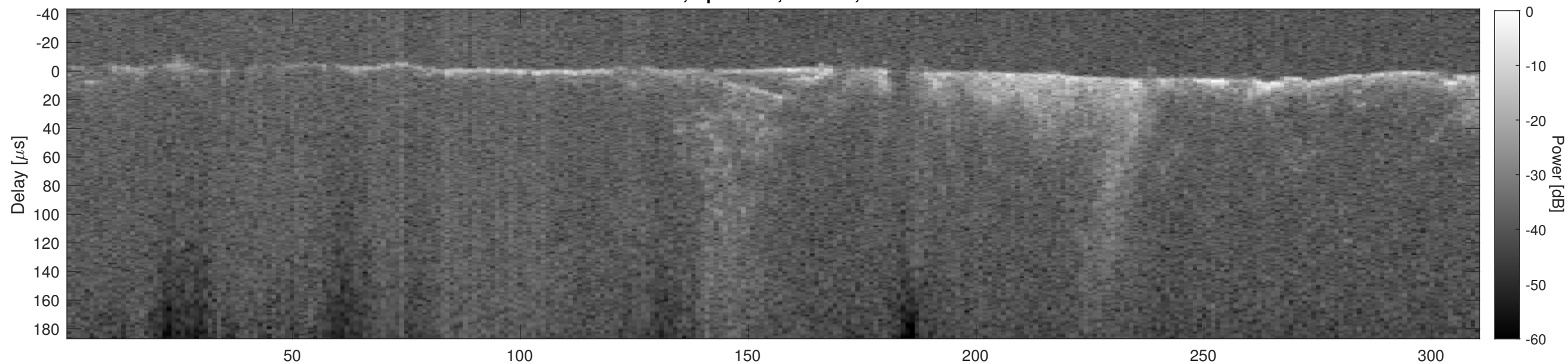
Orbit 3851, Cluttergram
