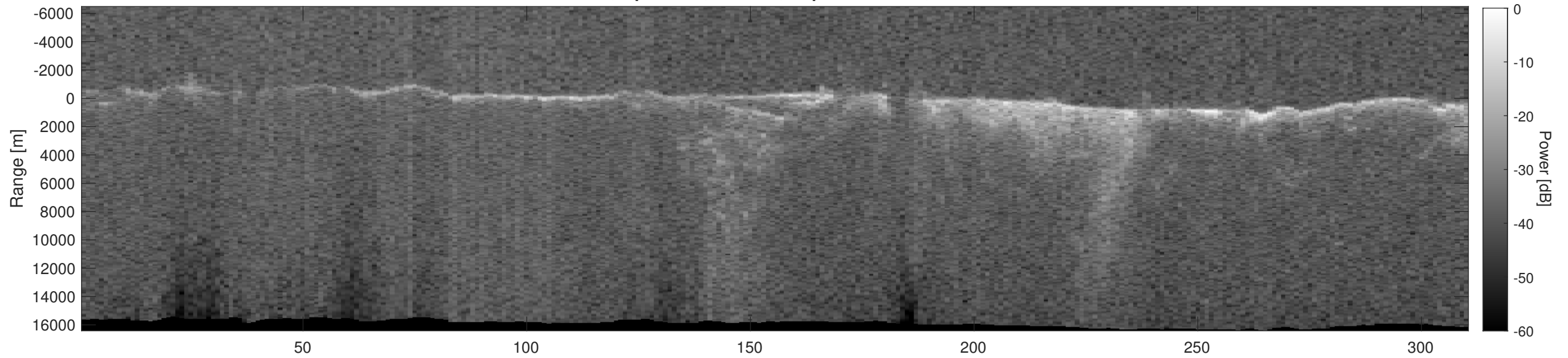
Orbit 3851, Depth-Corrected Cluttergram
