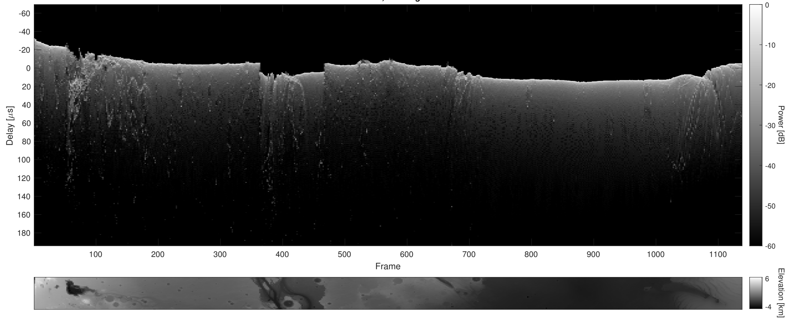
Orbit 3856, Cluttergram
