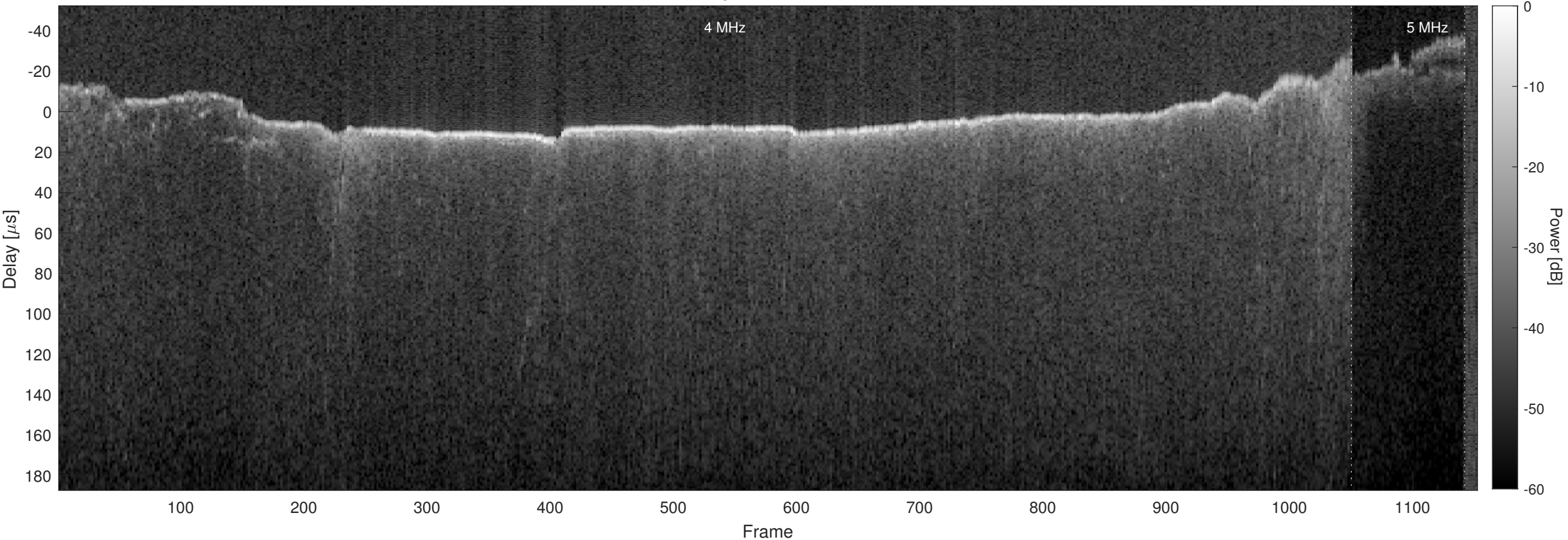
Orbit 3857, Chapman, Window, Channel 2
