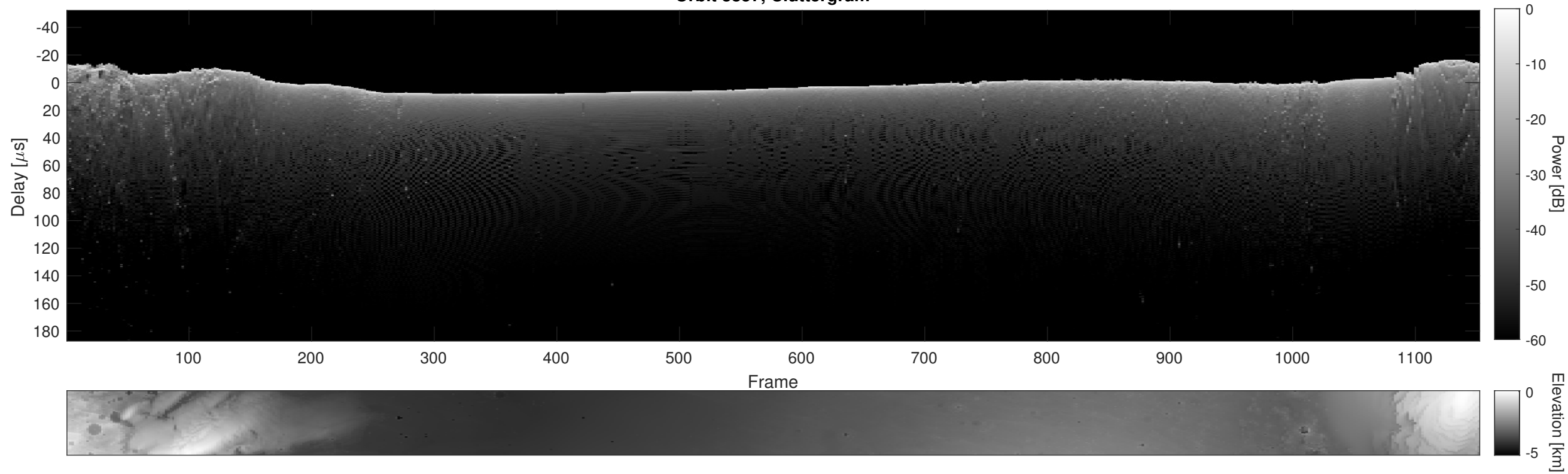
Orbit 3857, Cluttergram
