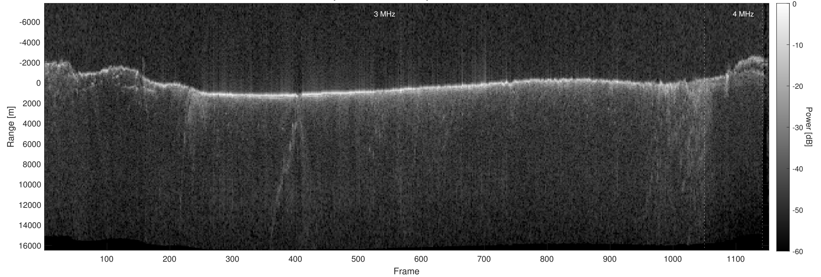
Orbit 3857, Optimized, Window, Depth-Corrected, Channel 2
