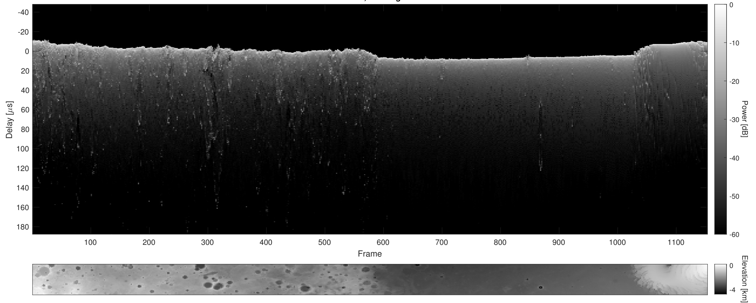
Orbit 3859, Cluttergram
