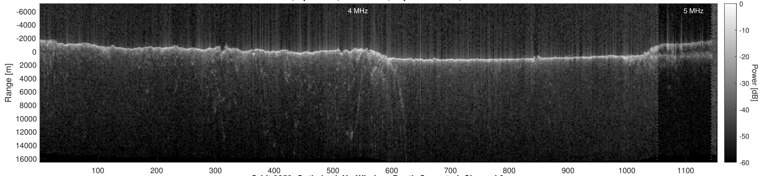
Orbit 3859, Optimized, No Window, Depth-Corrected, Channel 2
