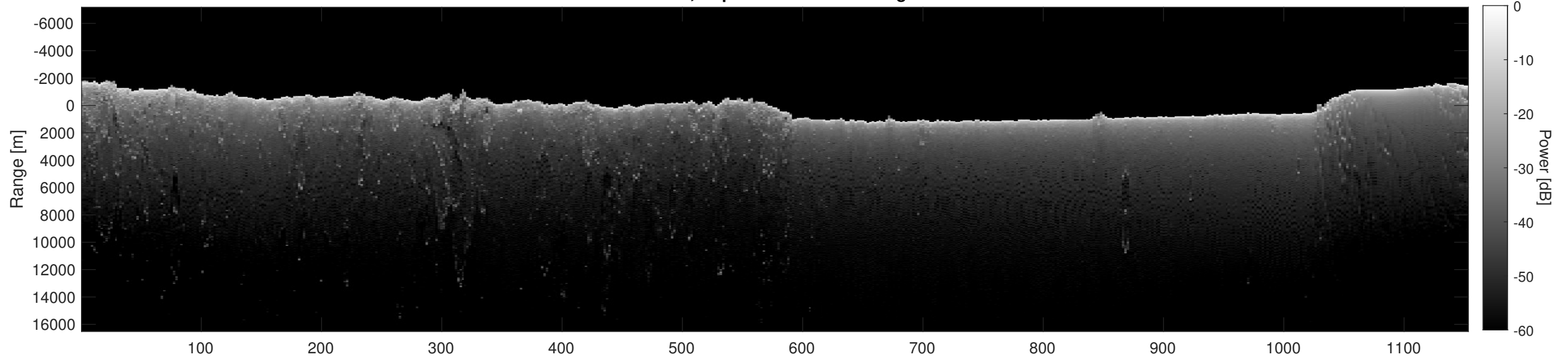
Orbit 3859, Depth-Corrected Cluttergram
