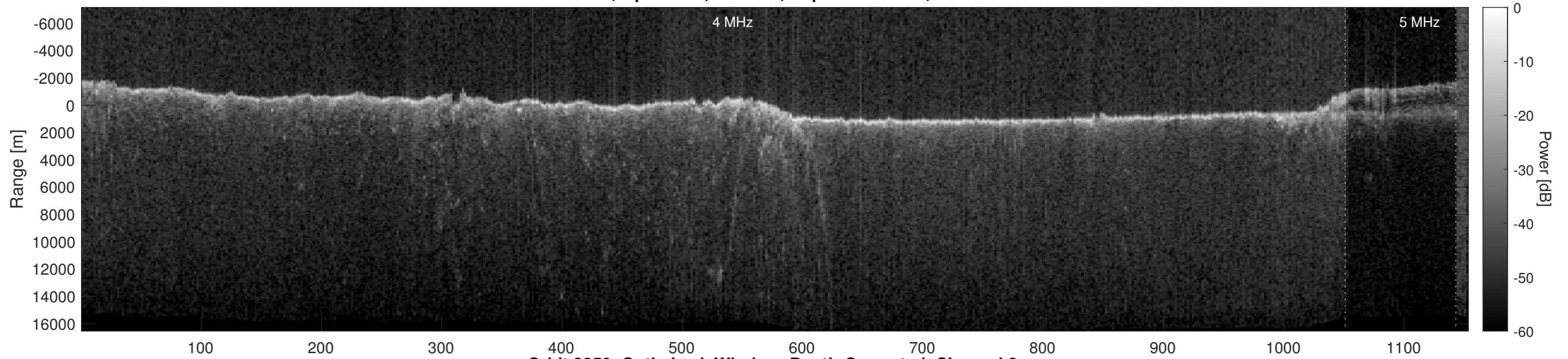
Orbit 3859, Optimized, Window, Depth-Corrected, Channel 2
