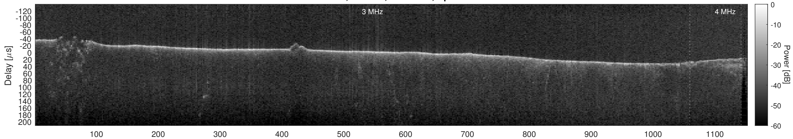
Orbit 3860, Cluttergram
