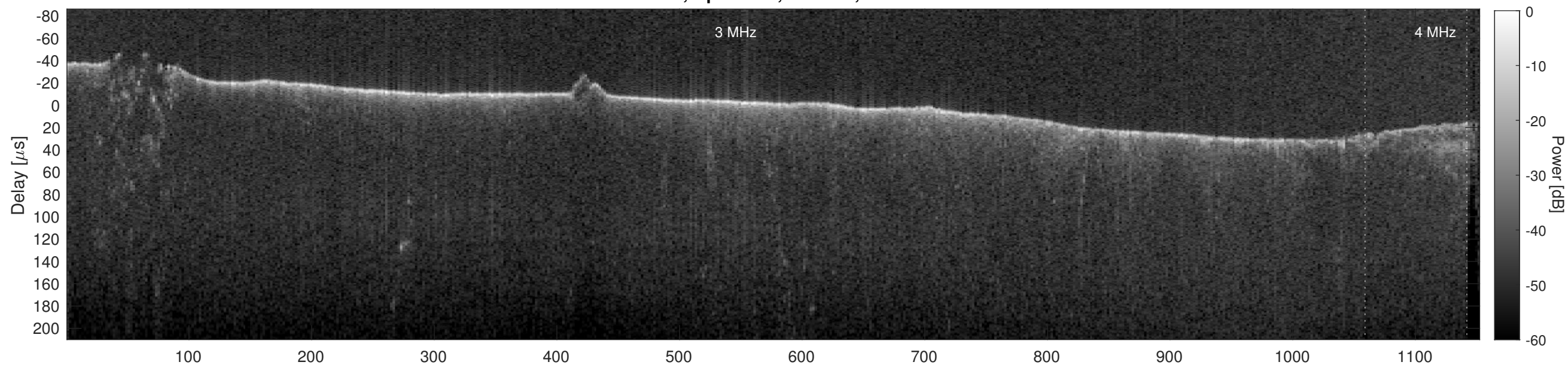
Orbit 3860, Cluttergram
